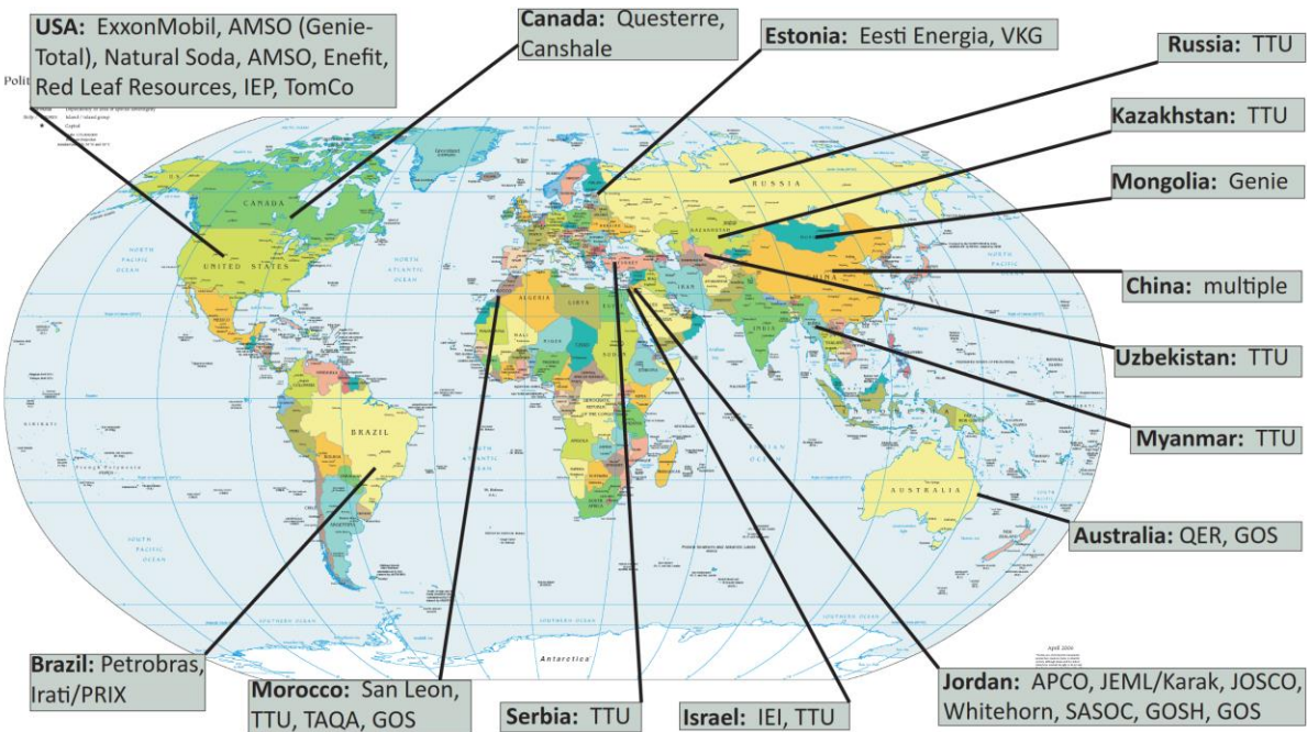
Figure 1: Oil shale projects around the world (Boak, 2014).
