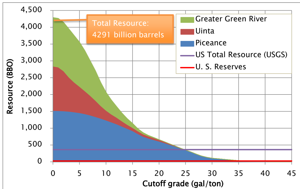
Figure 3: Oil Shale resource estimates for different grades of oil shale, from U.S. Geological Survey data (presented at the 32 nd Oil Shale Symposium).
