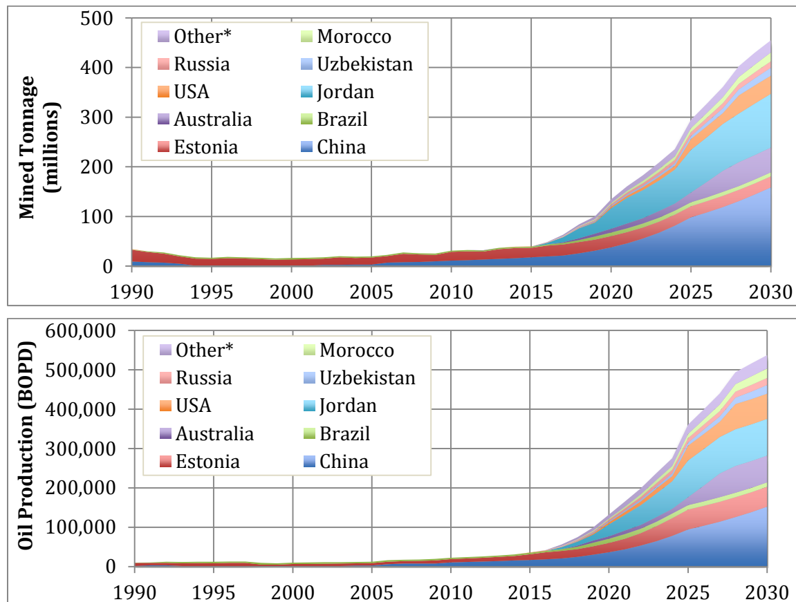
Figure 2: Current and projected quantities of mined oil shale and shale oil produced by pyrolysis. Much of the mined oil shale is burned directly to produce electricity.
