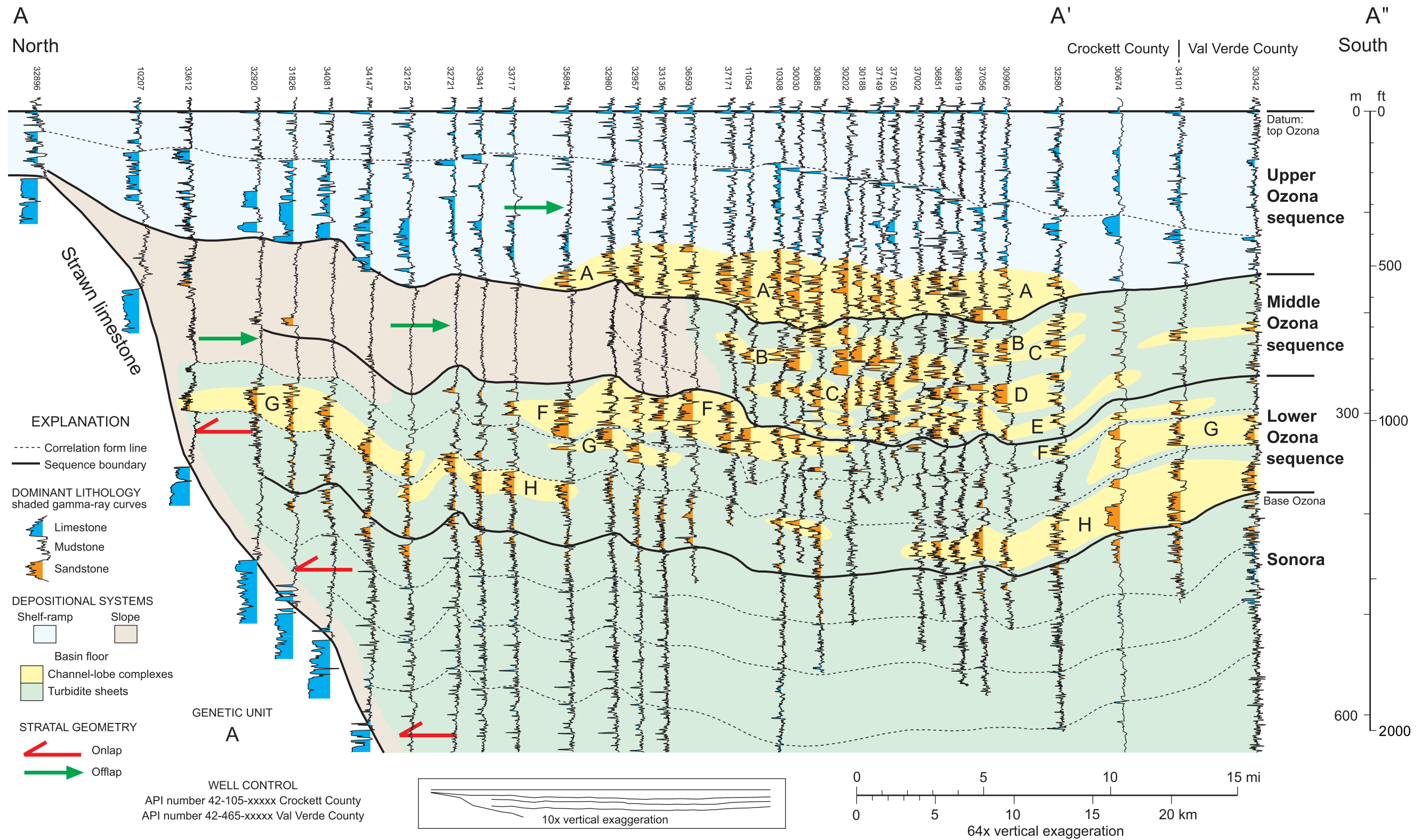
Datashare 31. North-south stratigraphic dip cross section AA' showing gamma-ray logs, lithologies, genetic units, depositional systems, sequences, and stratal geometries. The line of section is located in Figures 1 and 3.
